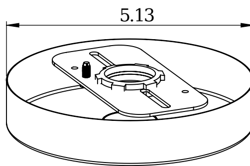
640-75 - 3/4" NPT CANOPY
