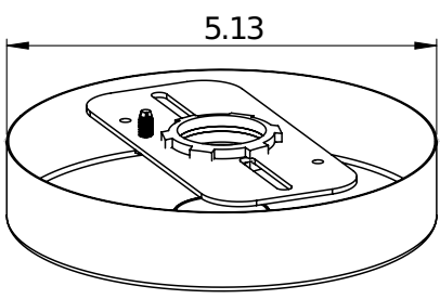
640-75 - 3/4" NPT CANOPY
