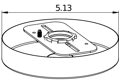
640-75 - 3/4" NPT CANOPY
