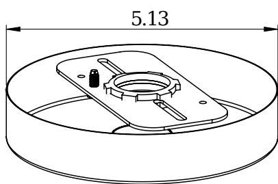
640-75 - 3/4" NPT CANOPY
