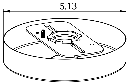
640-75 - 3/4" NPT CANOPY
