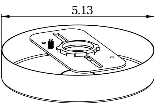
640-75 - 3/4" NPT CANOPY
