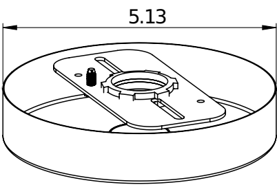
640-75 - 3/4" NPT CANOPY
