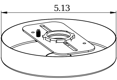
640-75 - 3/4" NPT CANOPY
