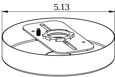
640-75 - 3/4" NPT CANOPY
