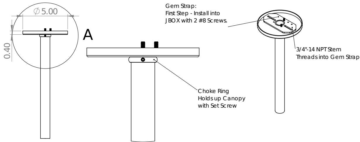
DETAIL A SCALE 1 : 2
